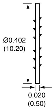
WASHER
